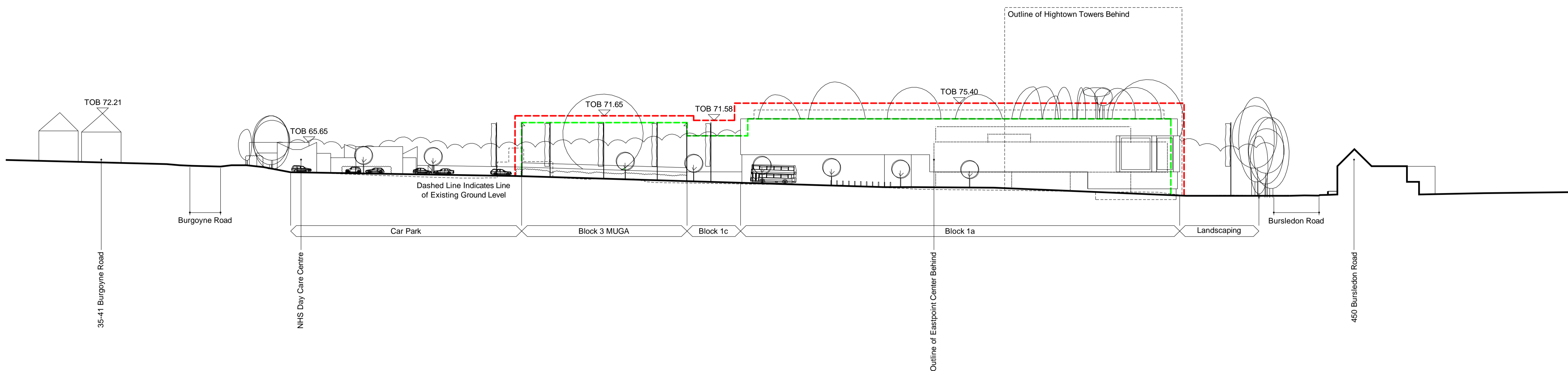
Proposed Section C-C Burgoyne Road to Bursledon Road Looking Southeast
