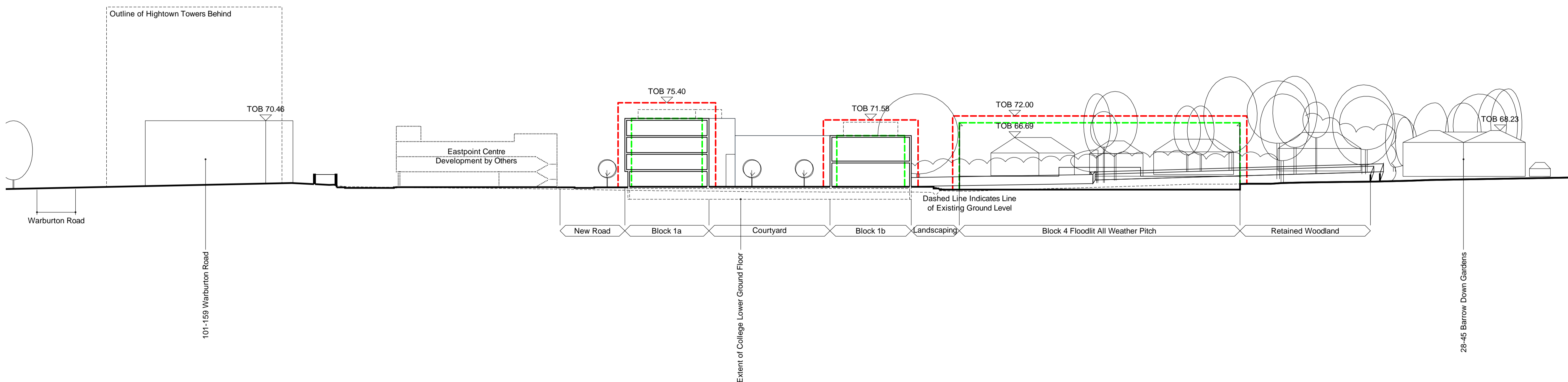
Proposed Section D-D Cross Section Through Site Looking Northeast
