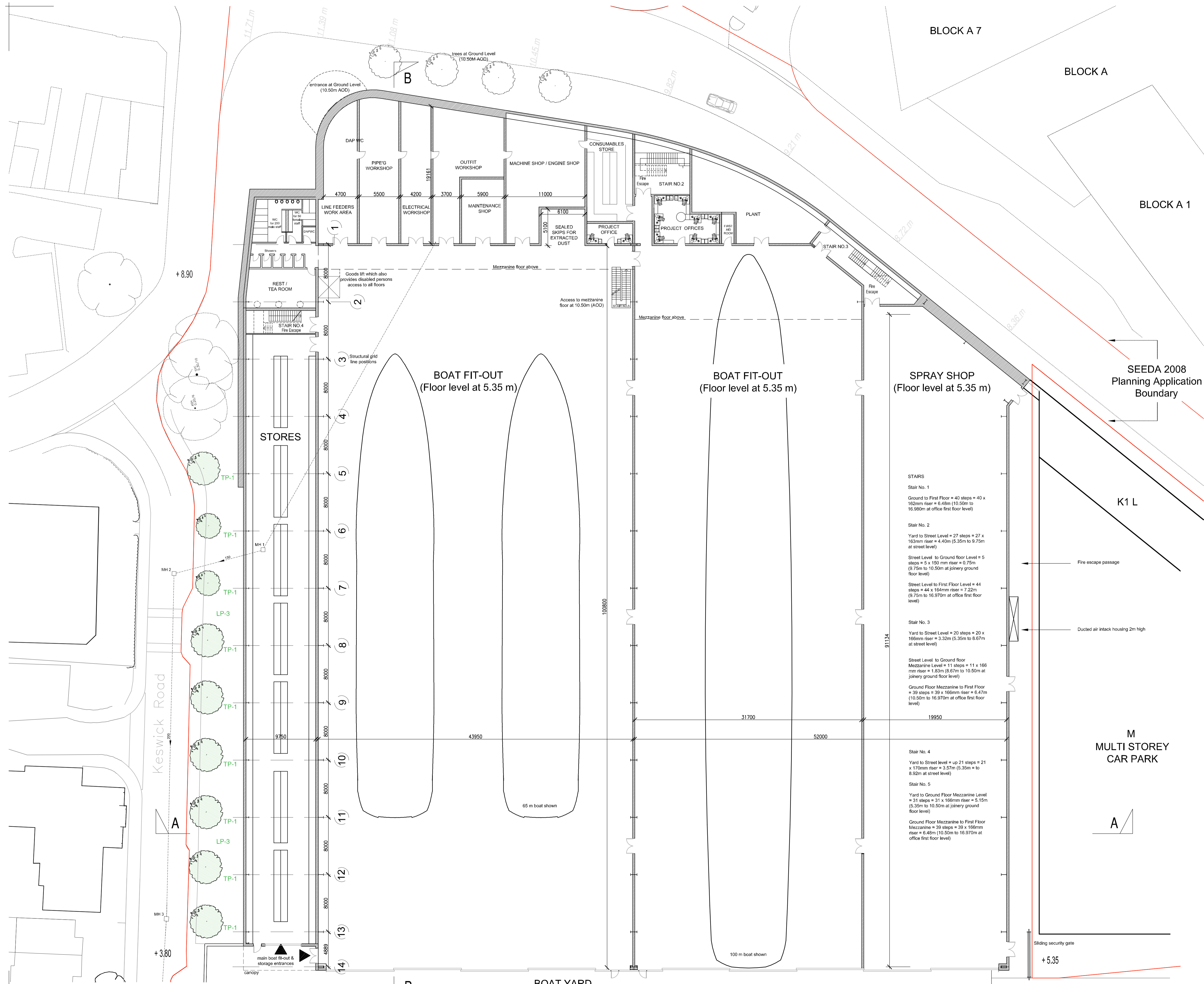
YARD LEVEL FLOOR PLAN @ 5.35 m (AOD)
