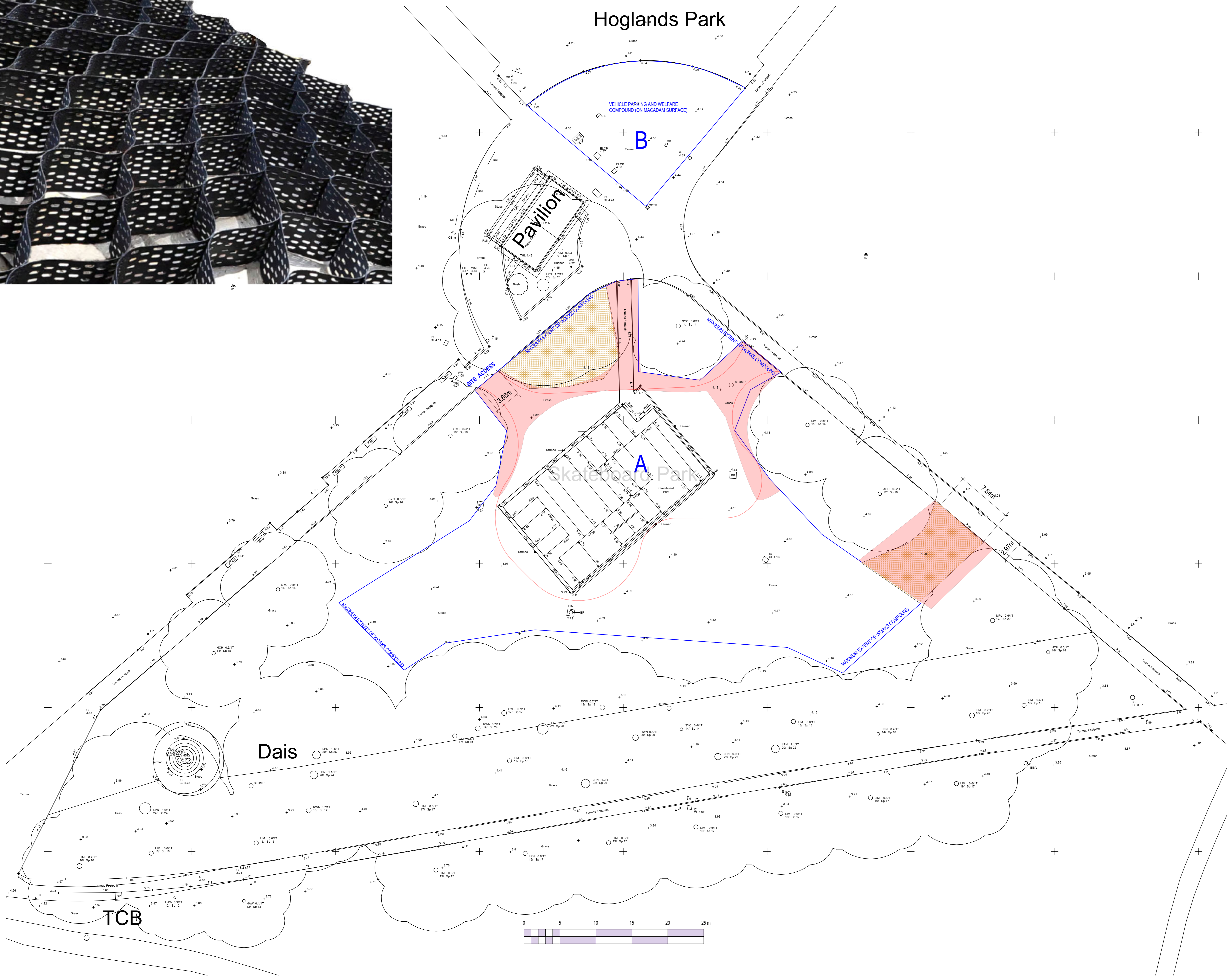
"CORE" TREE ROOT PROTECTION SYSTEM
